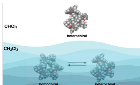
Homochiral-heterochiral switch in dichloromethane within a trinuclear circular Ti(IV)-based architecture
