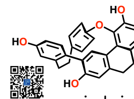
cavicularin
