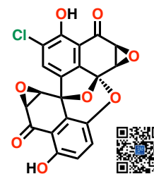
spiroxin A
