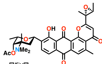
saptomycin H
