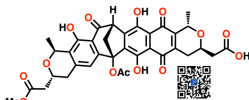
\beta -naphthocyclinone
