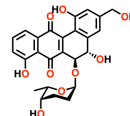
TAN-1085
