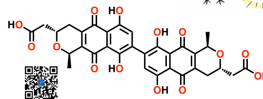
actinorhodin
