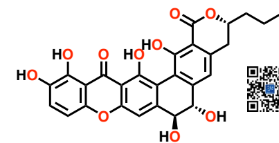
FD-594 aglycon
