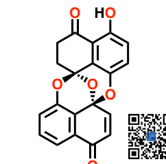
preussomerin EG 1
