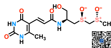
sparoxomycin A 2
